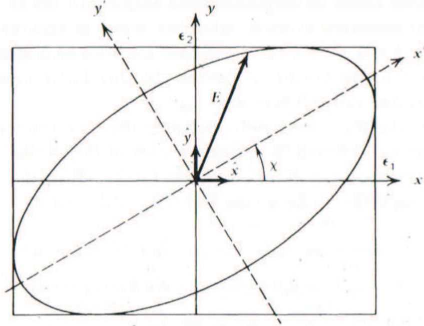
Figure 2.1: An ellipse traced out by the electric field of an electromagnetic wave at a certain location. Its propagation is in z direction, i.e., out of the page (Rybicki & Lightman (1979), page 63).
