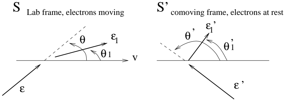
Figure 7.2: Notations used in analyzing inverse Compton scattering.
