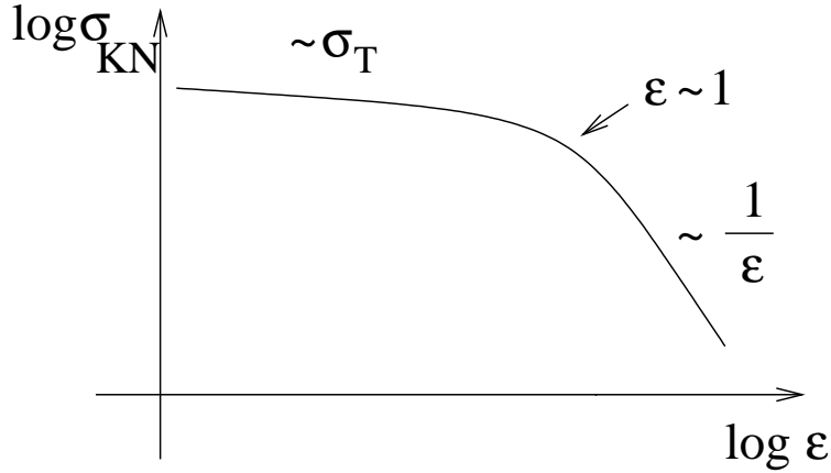
Figure 7.1: The Klein-Nishina cross section.
