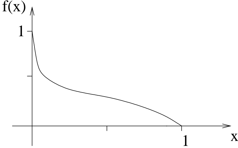
Figure 7.3: The function f(x) in the single electron inverse Compton spectrum.
